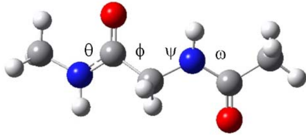
Fig. 1 Glycine dipeptide in its extended C5 conformation
