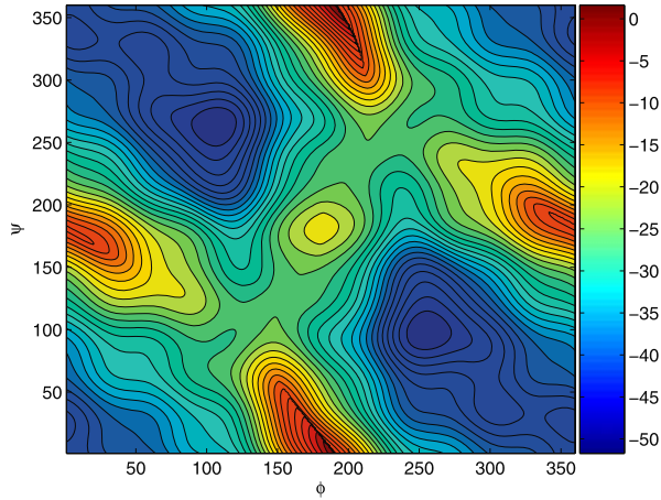
Fig. 4 Minimized potential energy landscape of the backbone angles
