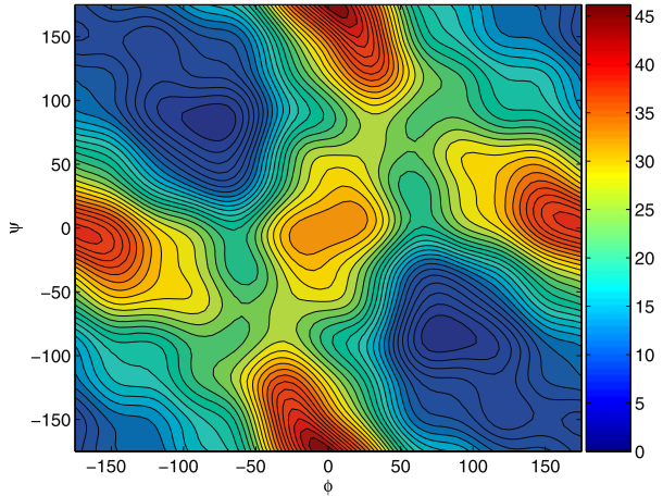
Fig. 2 Helmholtz free energy F(\phi, \psi) at T = 300 K
